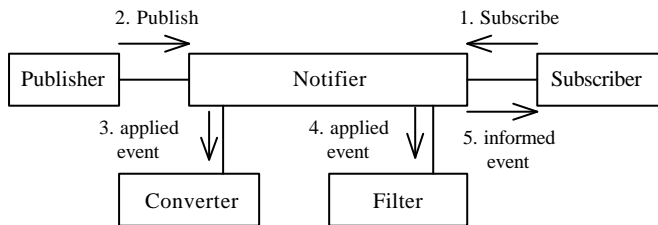
5. Collaboration Diagram
